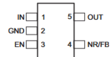
DCK Package 5-Pin SC70 Top View
